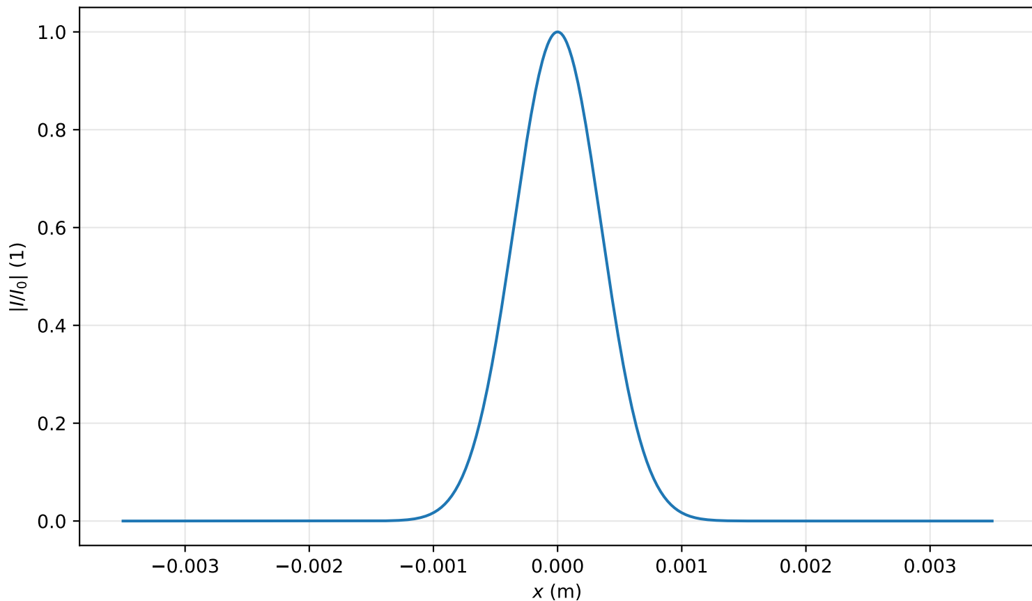
Intensity profile I(x, y = 0, z = 0.000m)/I_0 , P_{in}=0.5P_{cr} , artificial time
